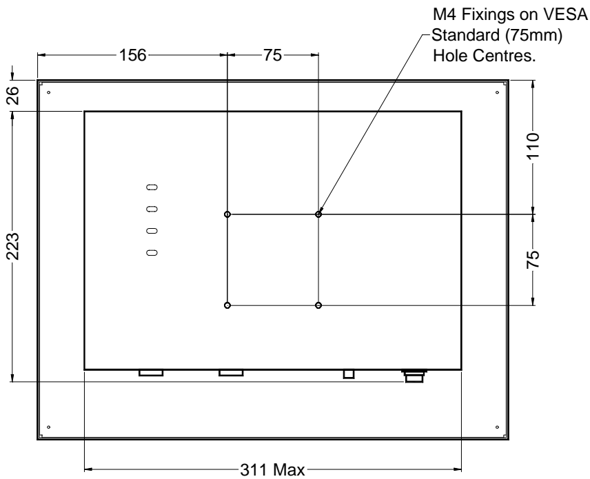
REAR VIEW
